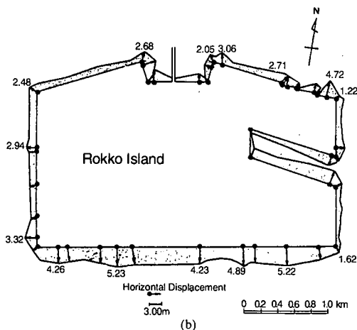
Fig.3 Displacement of quay walls at Port Island and Rokko Island.
