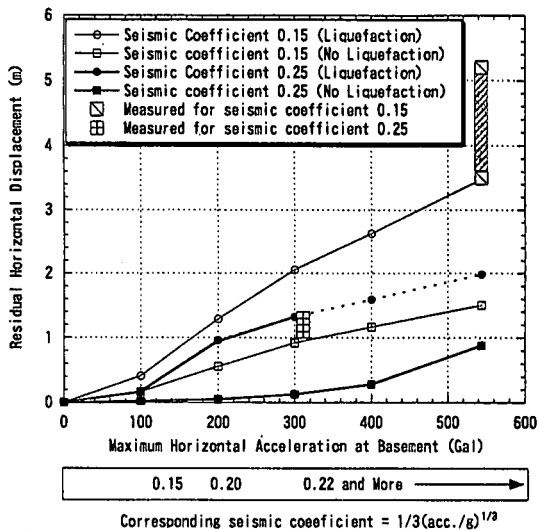
Fig.21 Horizontal displacement under various input acceleration levels.
