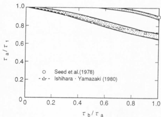
Fig.16 Reduction of liquefaction resistance under multiple shear (after Yoshimi, 1991)
