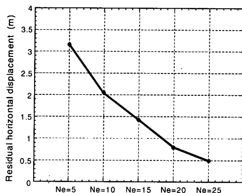
Fig.22 Horizontal displacement related to the equivalent SPT N values.
