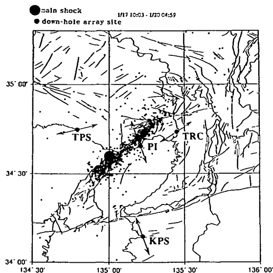
Fig.1 Location of down-hole array sites recorded around Osaka Bay and epicenters of the 1995 Hyogoken nambu earthquake (Summarized by Disas. Prev. Res. Inst.) (After Sato 5) )
