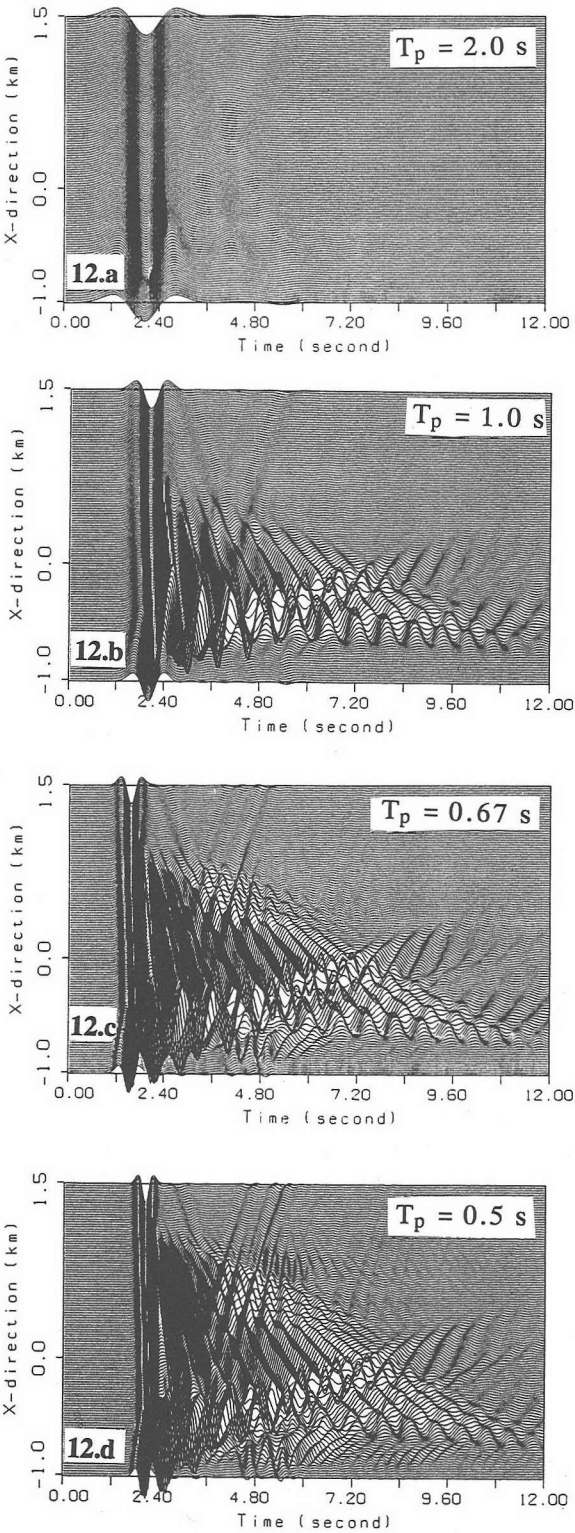
Fig.12 Alluvium surface displacement time histories due to SV-Ricker waves (horizontal components).
