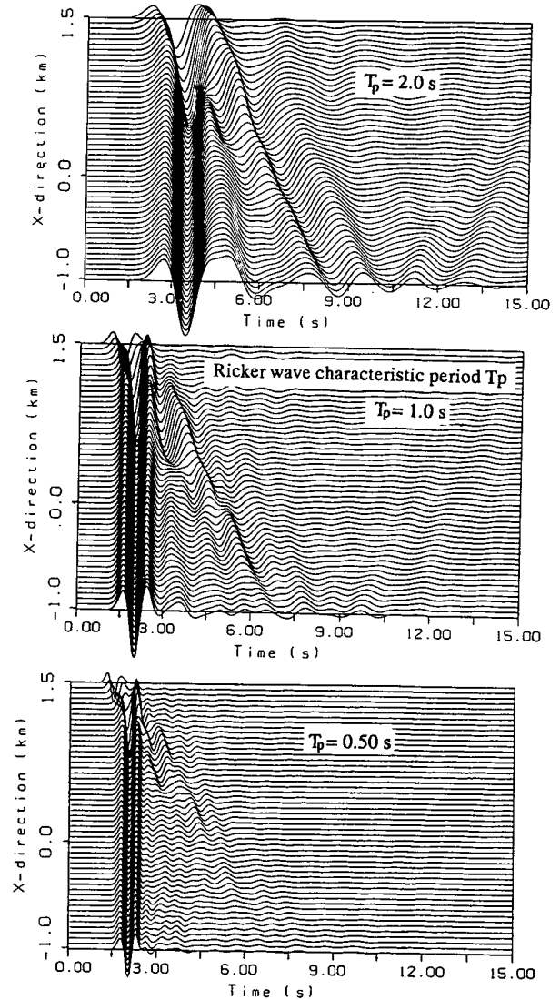
Fig.5 Displacement time histories due to SH-waves.
