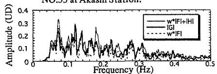
Fig.4.2 Fourier amplitude spectra of NO.69 at Monument Station.
