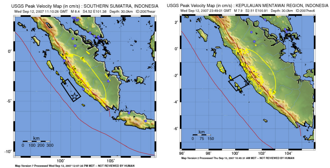
Fig.4.12 Estimated maximum ground velocities by USGS for M8.4 and M7.9 events
