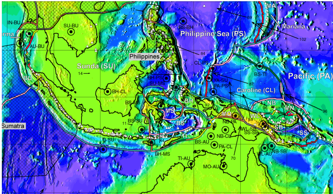
Fig.3.1 Major tectonic plates and platelets
