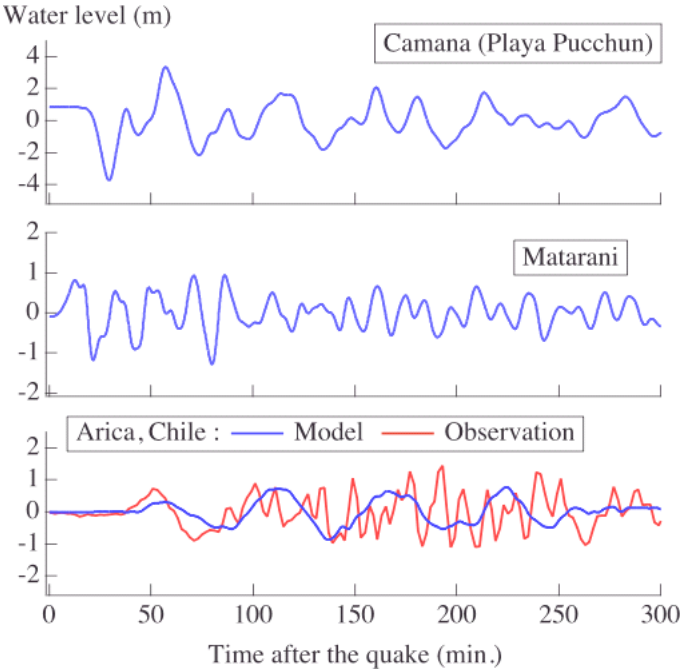
Figure 6.15 Computed and observed tsunami waveforms.
