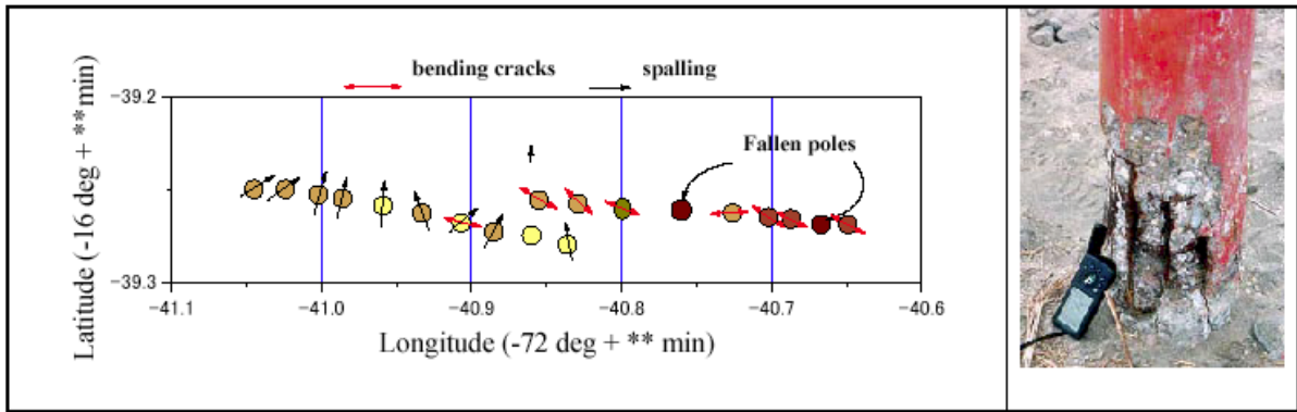
Figure 6.21 Spalled and cracked utility poles
