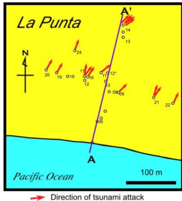
Figure 6.20 Possible directions of tsunami surge.
