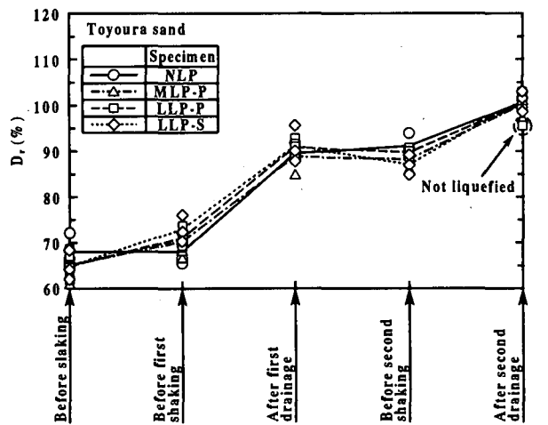
Fig. 7 Variation of D_r of each specimen before slaking, before first shaking, after first drainage, before second shaking and after second drainage (Toyoura sand).
