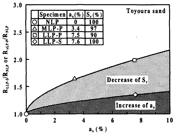
Fig. 5 Relationship between liquefaction resistance ratio, R_{LLP-S}/R_{NLP} or R_{XLP-P}/R_{NLP} area ratio of quick lime pile a_s (Toyoura sand).
